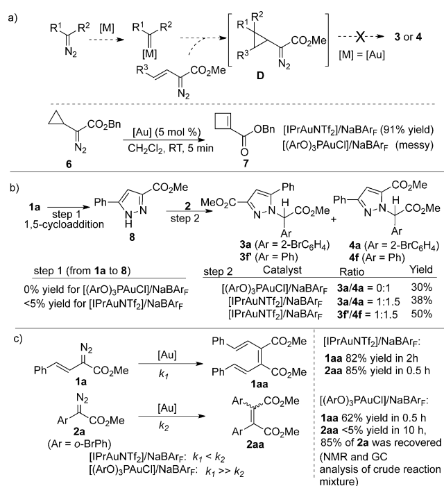
Scheme 3. Control experiments.
